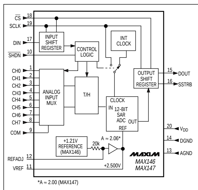
Figure 3. Block Diagram
