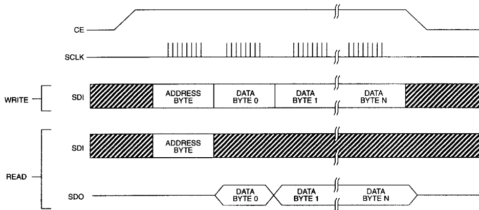
Figure 8. SPI MULTIPLE-BYTE BURST TRANSFER
