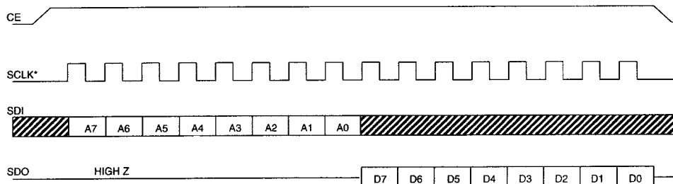
Figure 7. SPI SINGLE-BYTE READ
