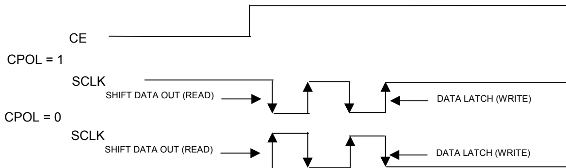
Figure 5. SERIAL CLOCK AS A FUNCTION OF MICROCONTROLLER CLOCK POLARITY (CPOL)
